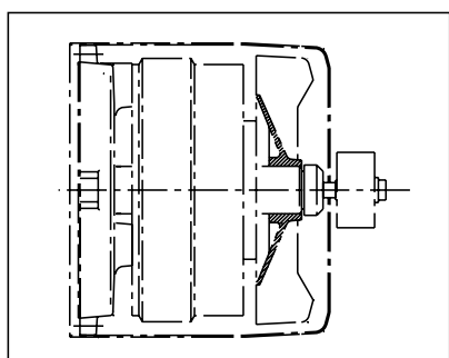
Special version Type of cooling IC 411, self-ventilated with built-on brake and incremental encoder
